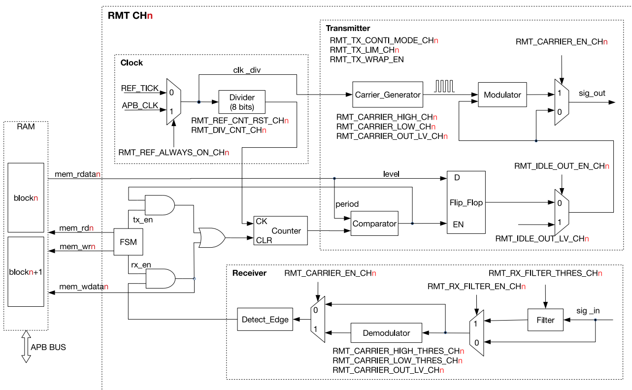
Figure 31-1. RMT Architecture
