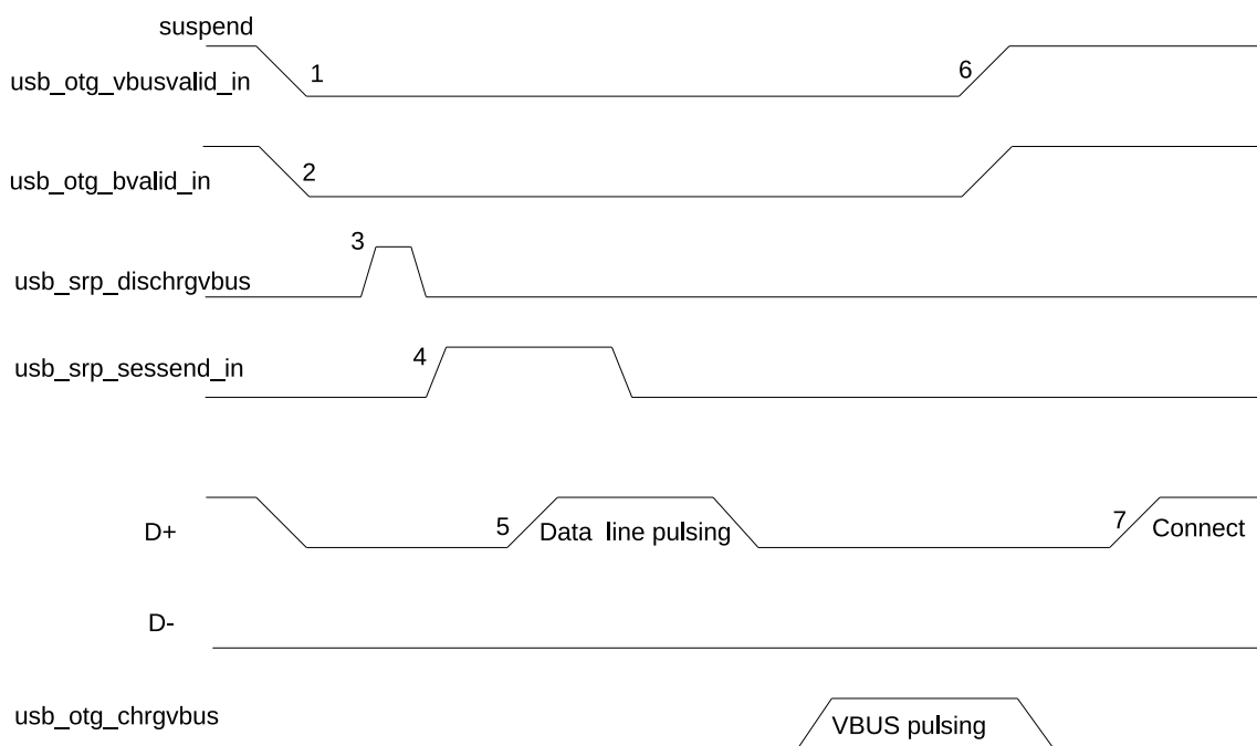
Figure 28-8. B-Device SRP
